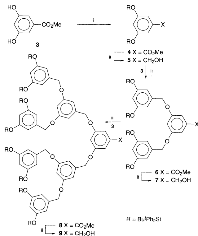
Scheme 1 Reagents: i, Bu t Ph 2 SiCl, imidazole, DMF; ii, LiAlH 4 , THF; iii, EtO 2 CN=NCO 2 Et, PPh 3 , THF
