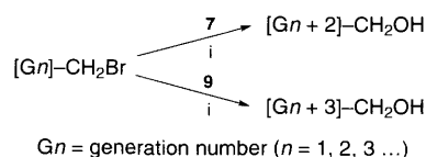
Scheme 2 Reagents and conditions: i, KF, 18-crown-6, acetone, reflux, 24 h
